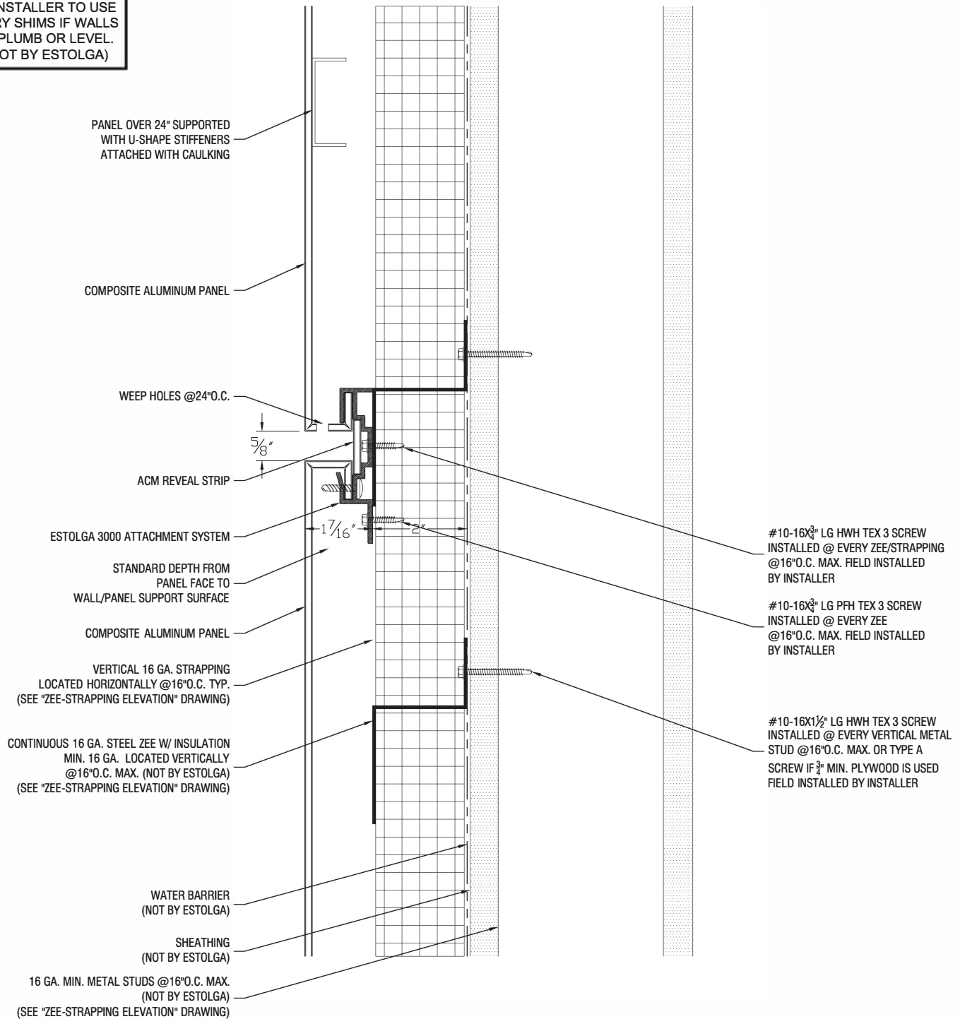
Typical Horizontal Joint Detail
